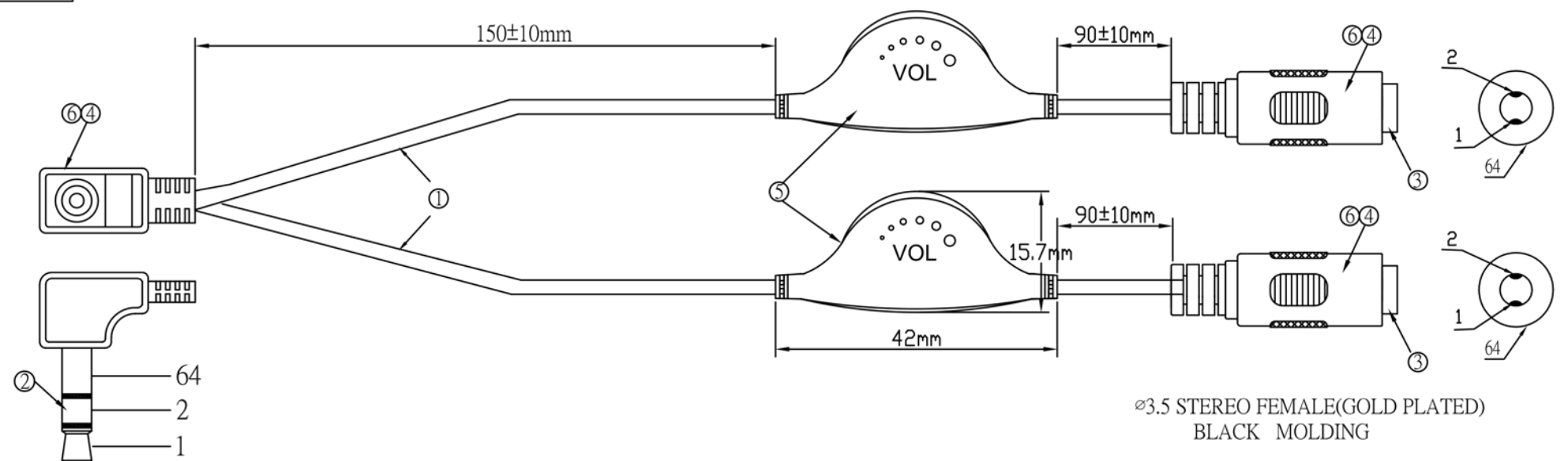
ø3.5 STEREO MALE(GOLDPLATED) BLACK MOLDING
