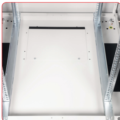
Base plate with cable feed
