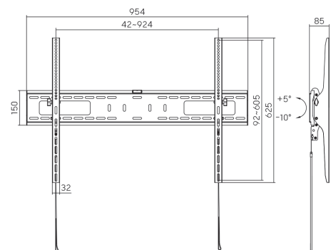
Dimensions (mm)
